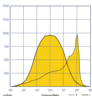
A6: 60° Asymmetrical Optic
