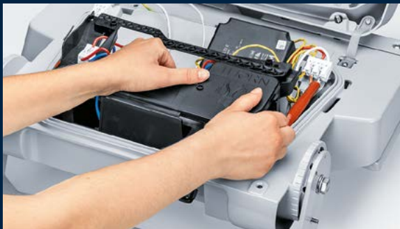
Step 3: Open the gear housing cover to access the connectors for main supply and controls.
