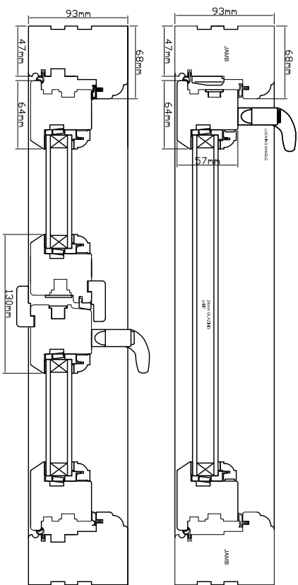
TIMBER WINDOW CASEMENT JAMB AND TRICKLE VENT DETAILS
