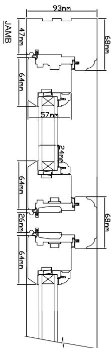
TIMBER WINDOW CASEMENT JAMB AND MULLION DETAIL
