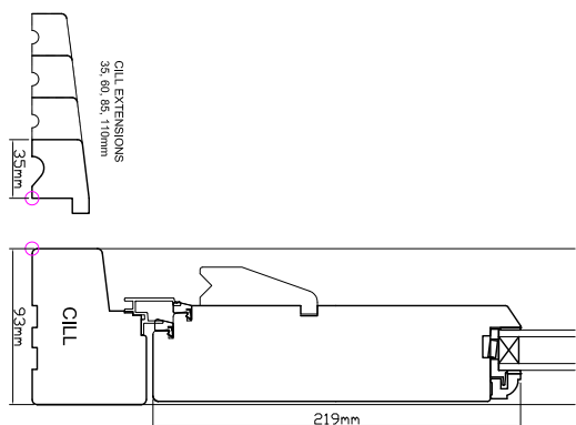
TIMBER DOOR JAMB AND DETAIL
