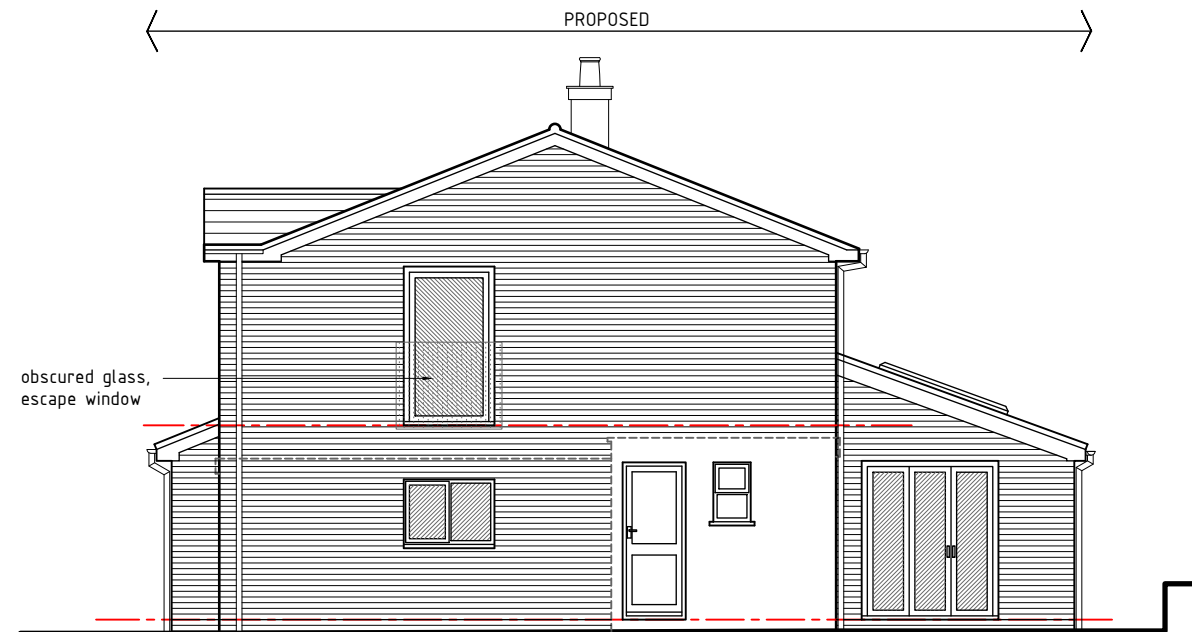
Side-01 Elevation 1:100
