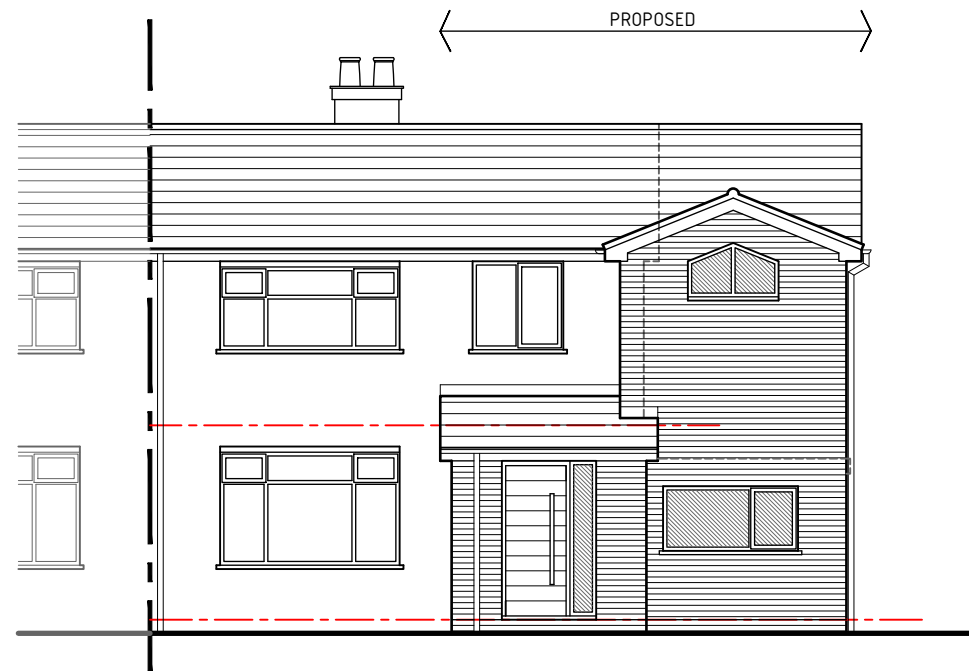
Front Elevation 1:100
