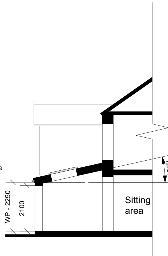
Typical Section 1:100
