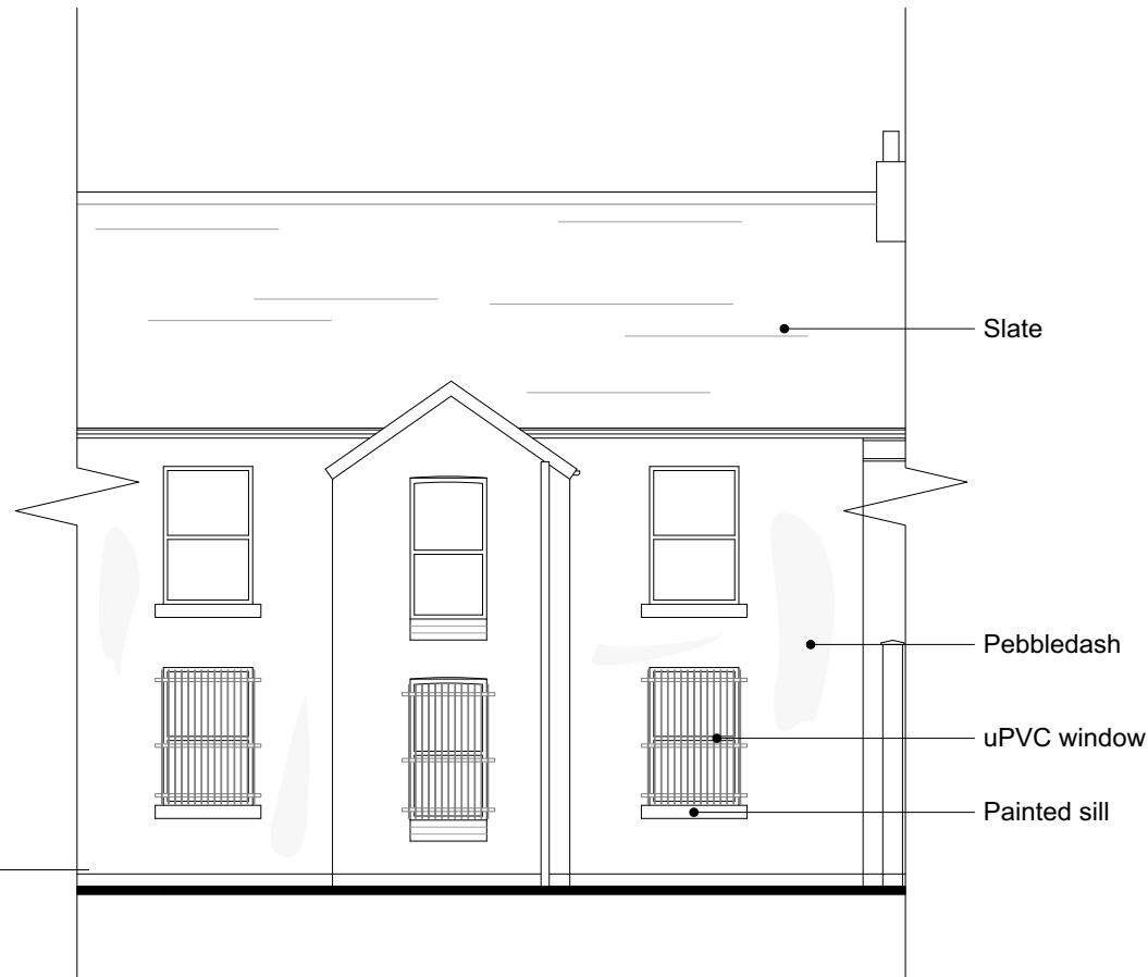
Existing Rear Elevation 1:100 View A
