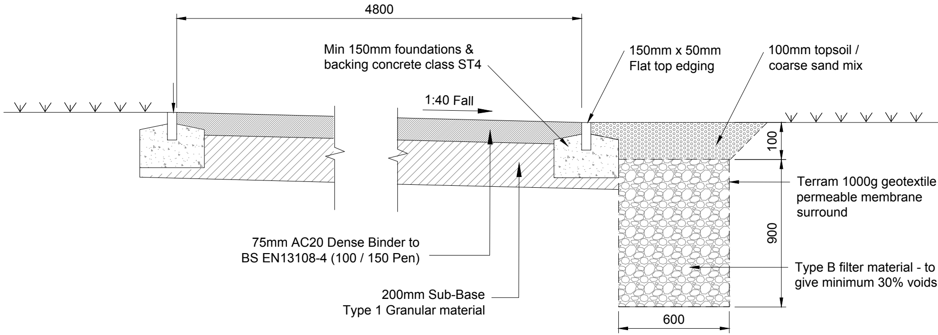
PROPOSED ACCESS ROAD
