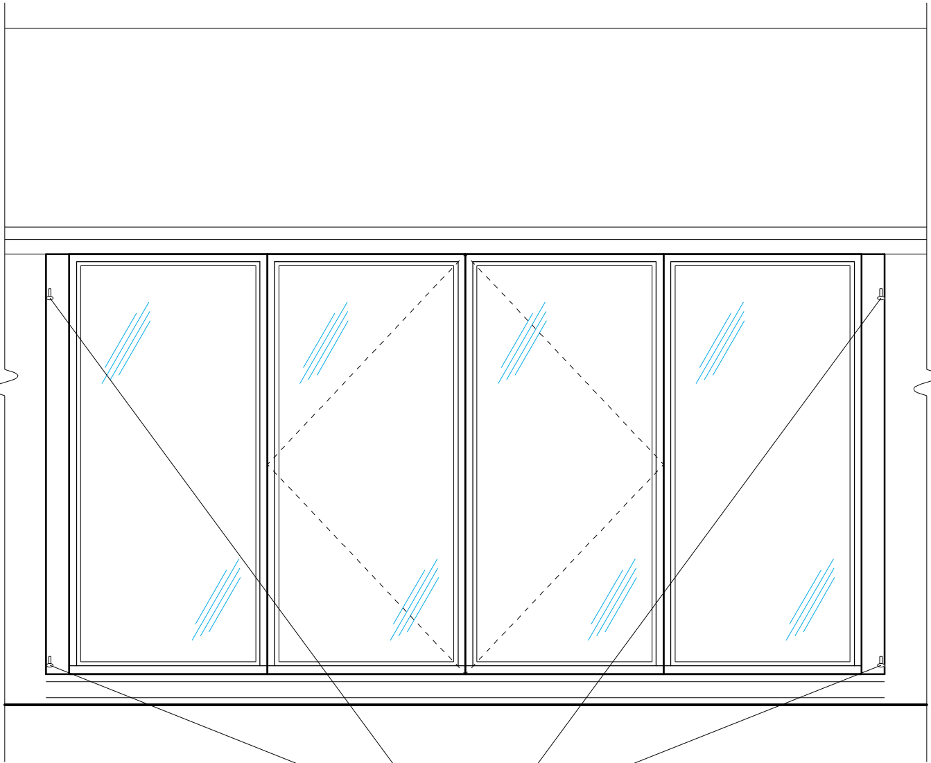
Proposed Doors/Glazed Panels Coach House 1:25
