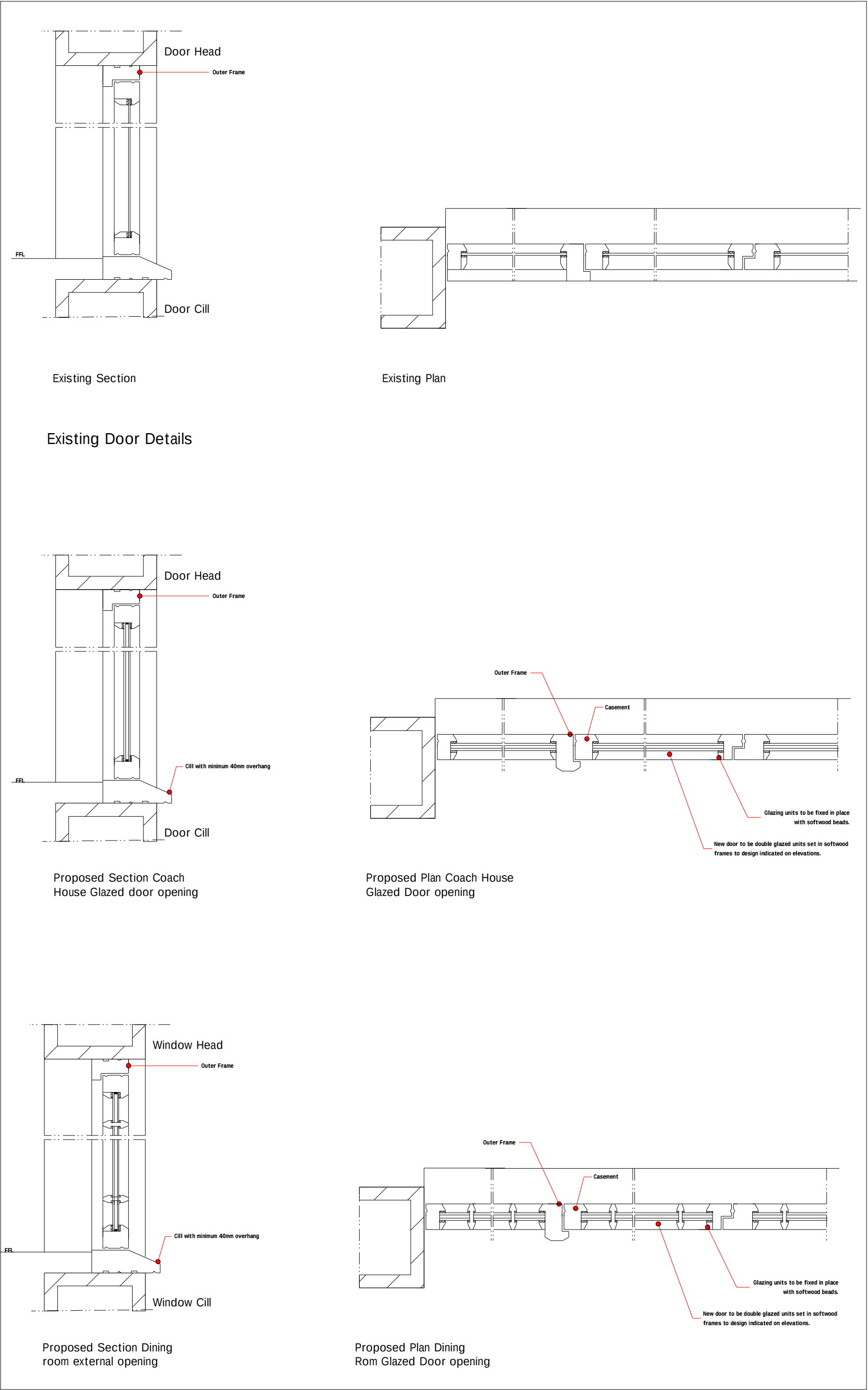
Proposed Door Detail 1:10
