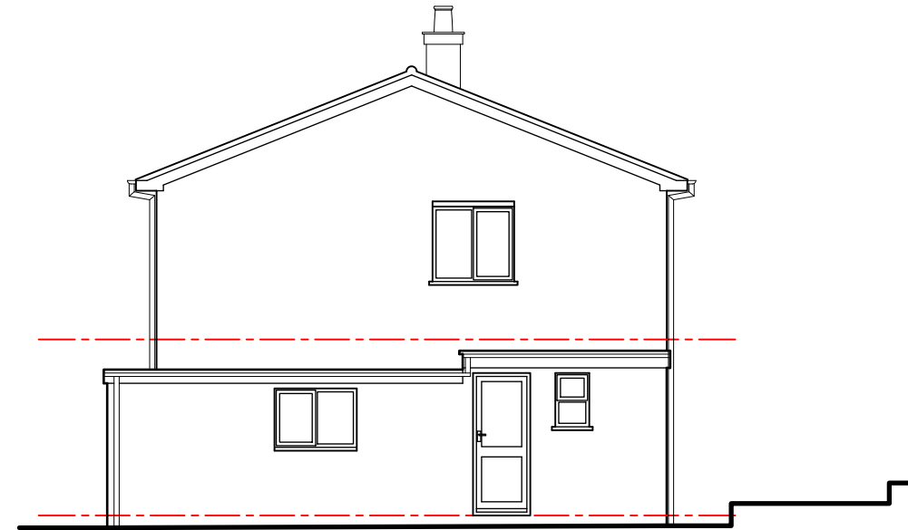
Side-01 Elevation 1:100
