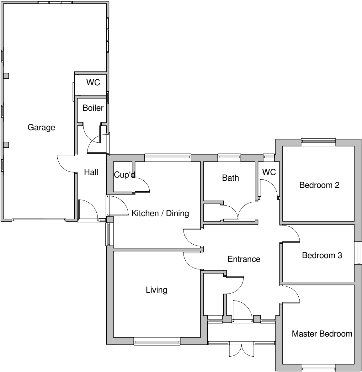
Ground Floor 1 : 100
