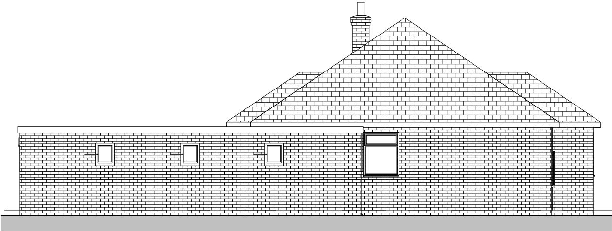
Side Elevation 1 : 100
