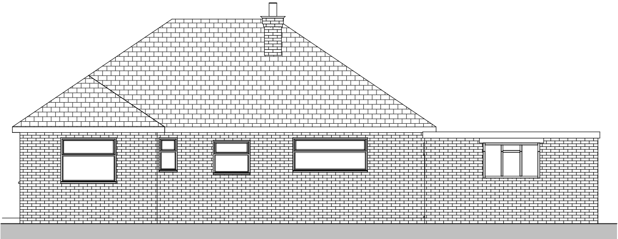
Rear Elevation 1 : 100
