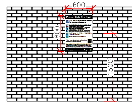
WALL MOUNTED Sign Type 2 600mm x 800mm
