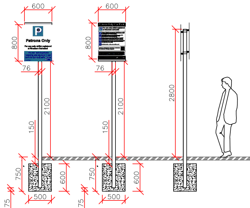
POLE MOUNTED Sign Type 1/2 600mm x 800mm
