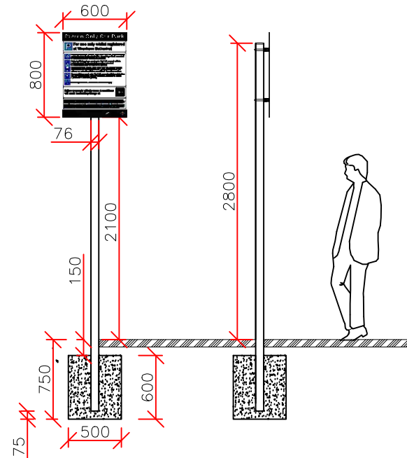
POLE MOUNTED Sign Type 2 600mm x 800mm
