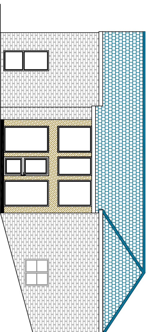
NORTH ELEVATION Scale 1 / 100
