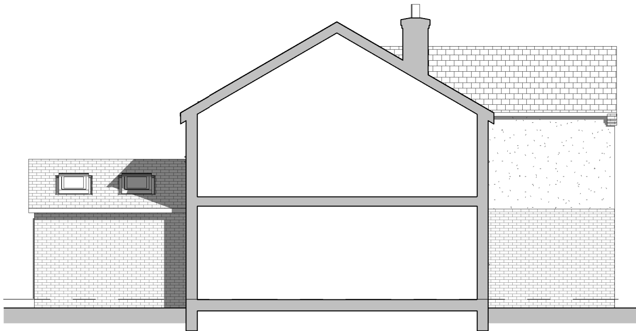
Side Elevation 1 : 100
