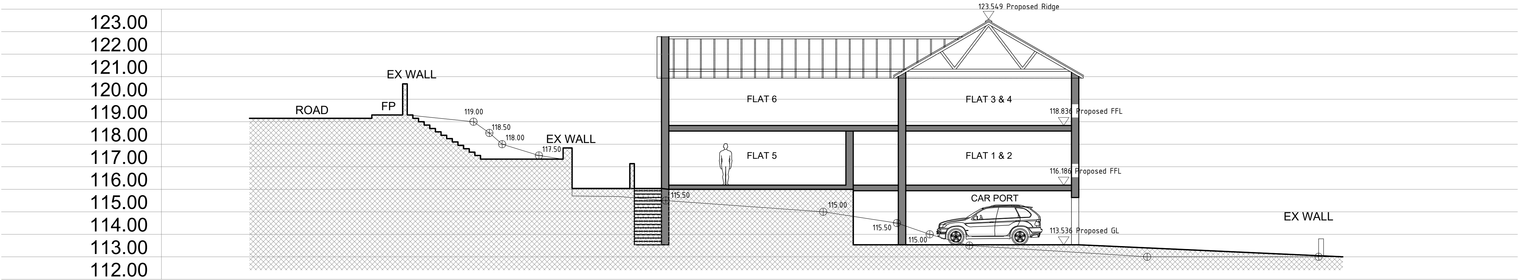
Section A-A as Proposed
