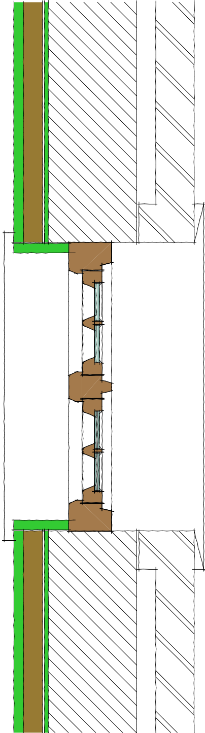
TYPICAL SECTIONS SCALE 1.10
