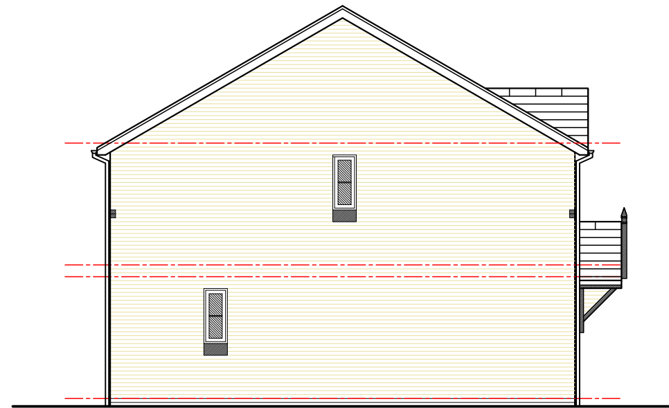
Side-01 elevation
