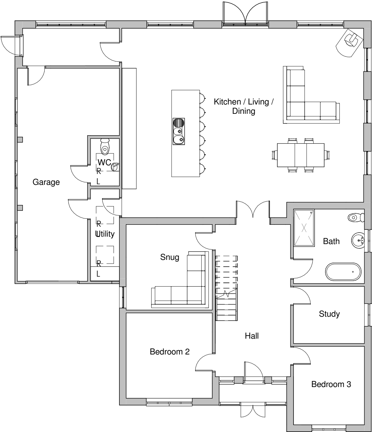
Ground Floor 1 : 100
