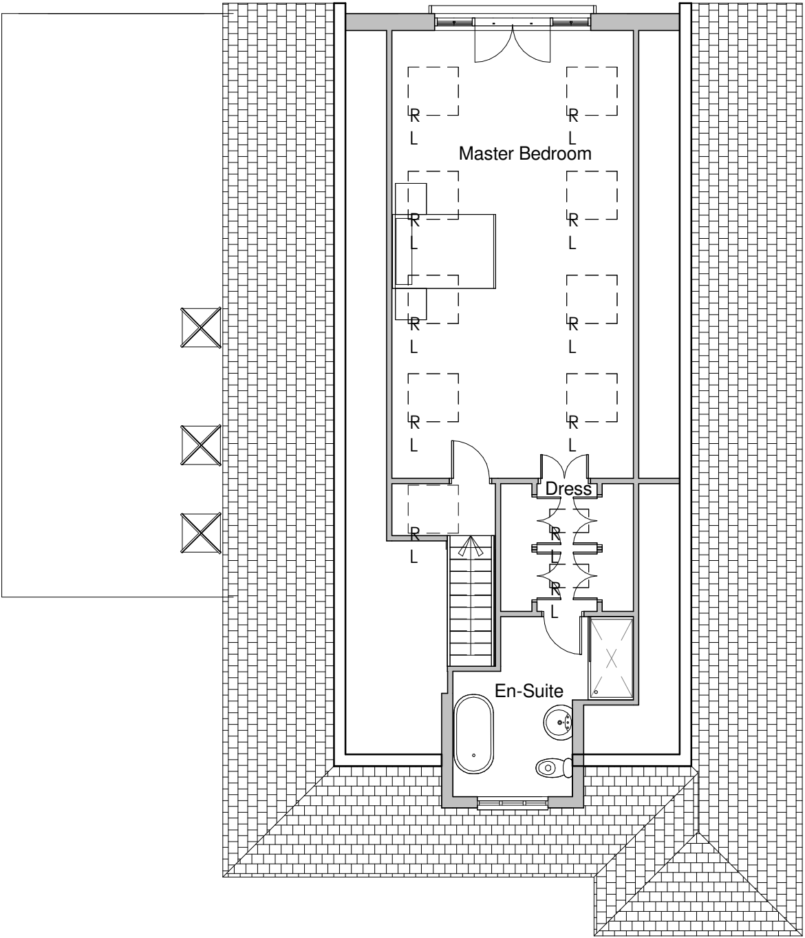
First Floor 1 : 100
