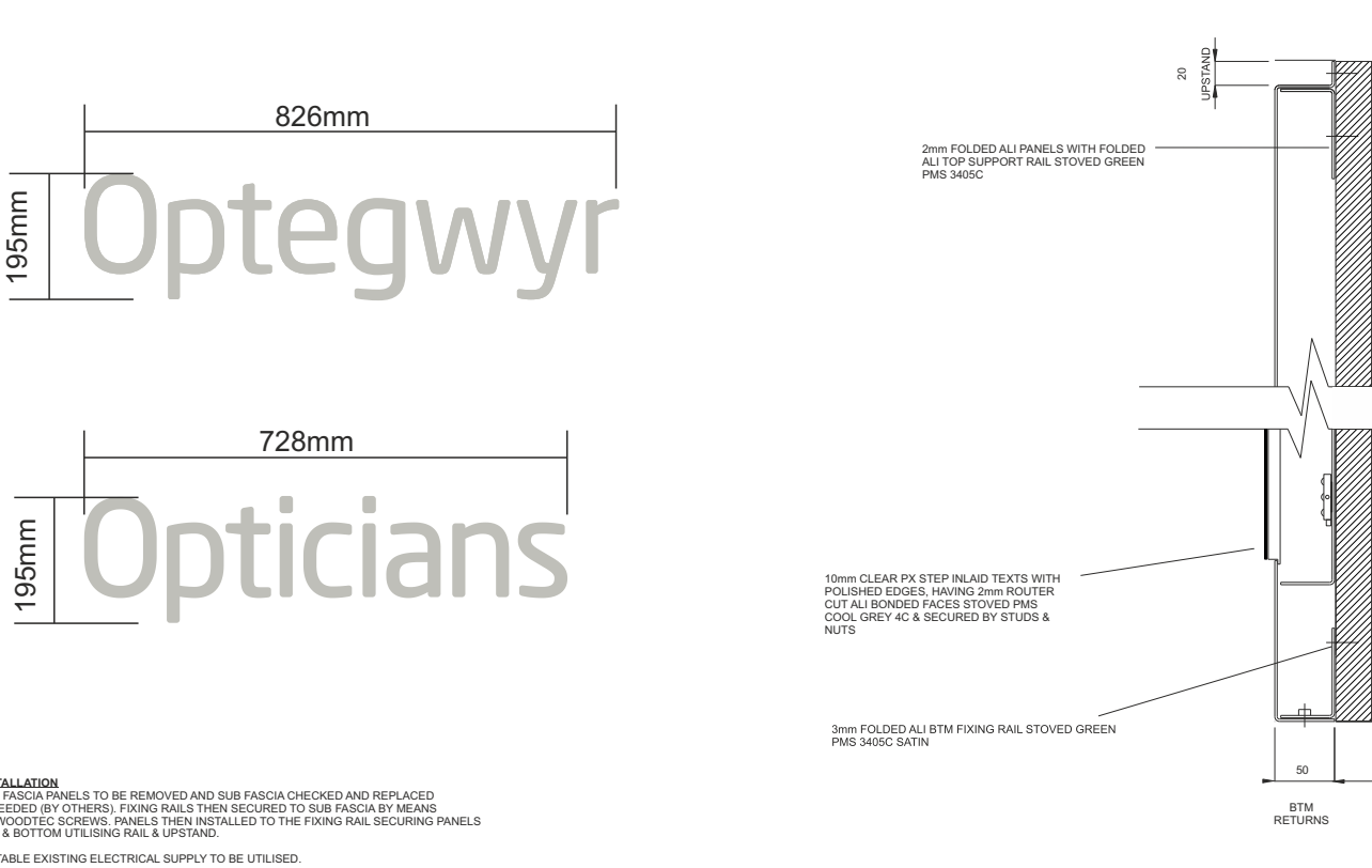
Internally Illuminated Fascia Descriptor Sign Detail
