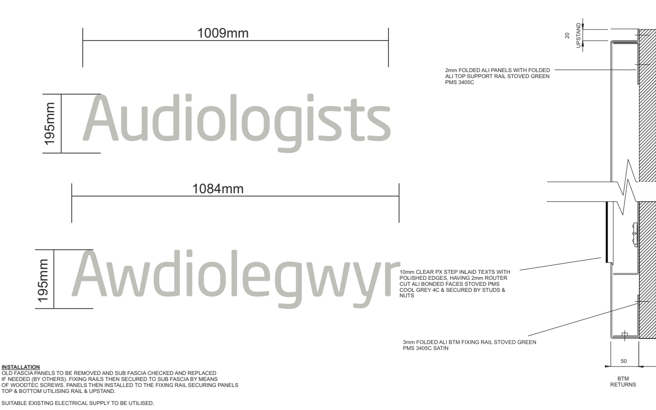
Internally Illuminated Fascia Descriptor Sign Detail
