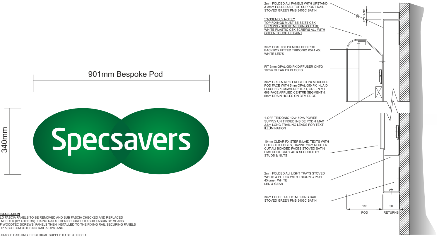
Internally Illuminated Fascia Pod Detail
