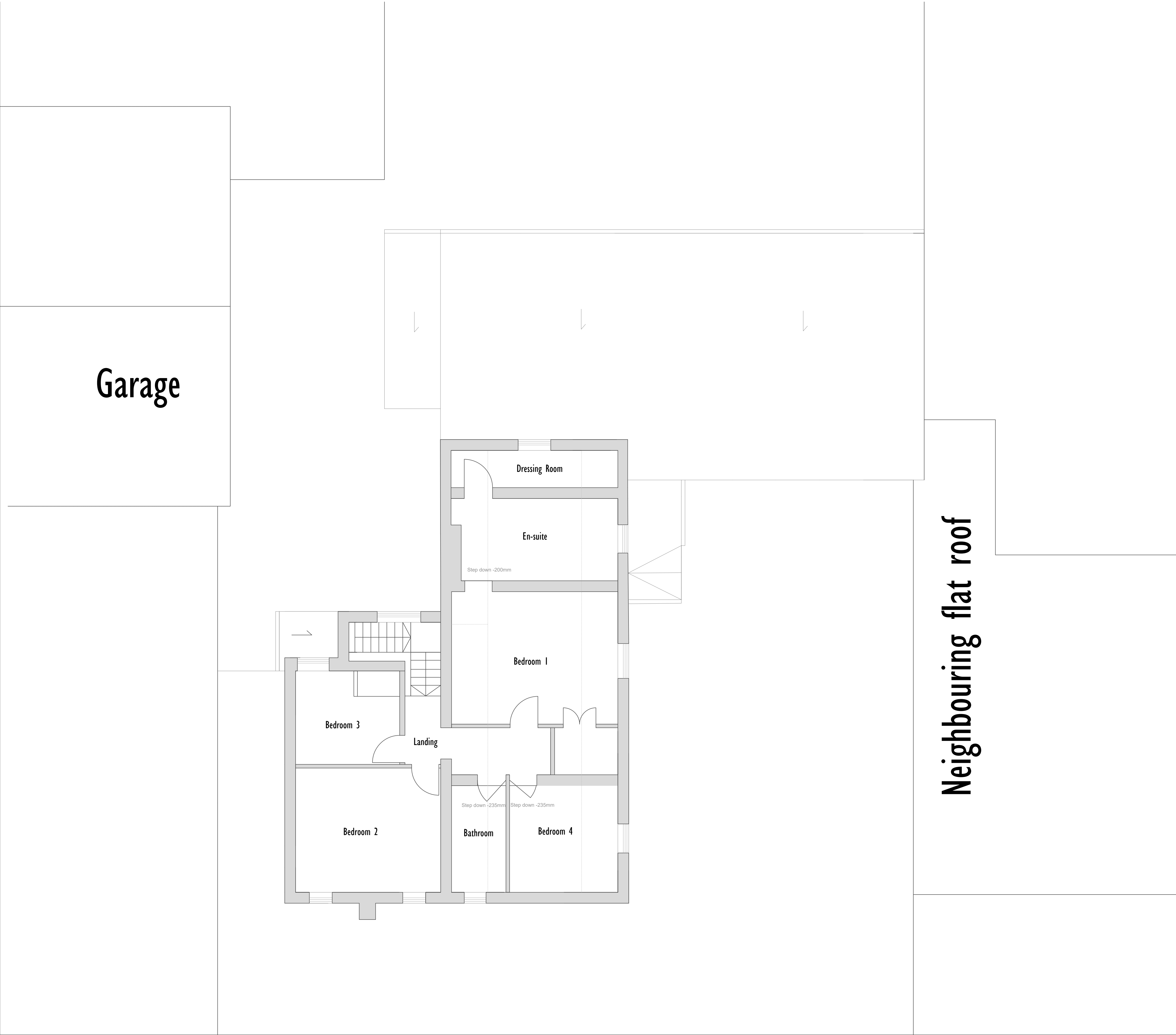
First Floor Plan ( 1:50)
