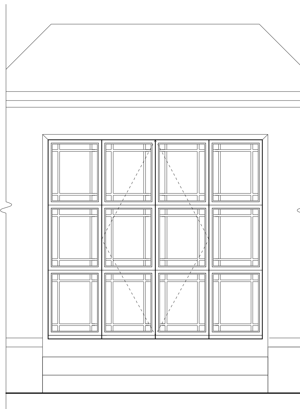
Proposed Dining Room Doors and Glazed Pannels - External View
