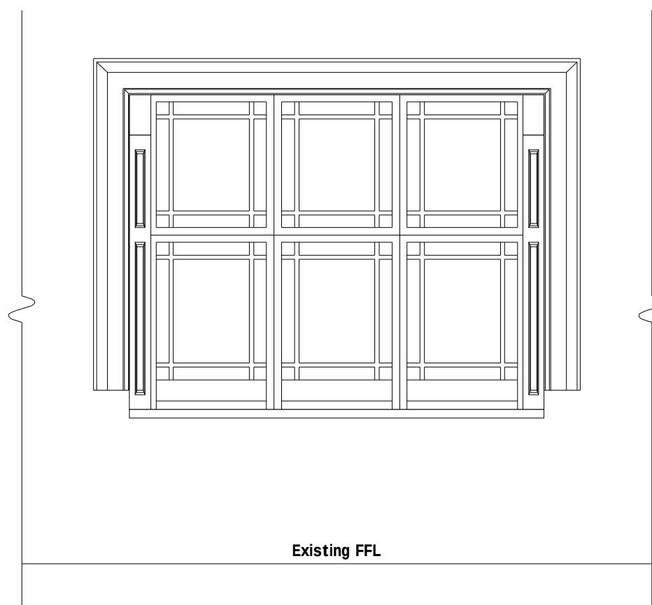
Existing Opening - Internal View
