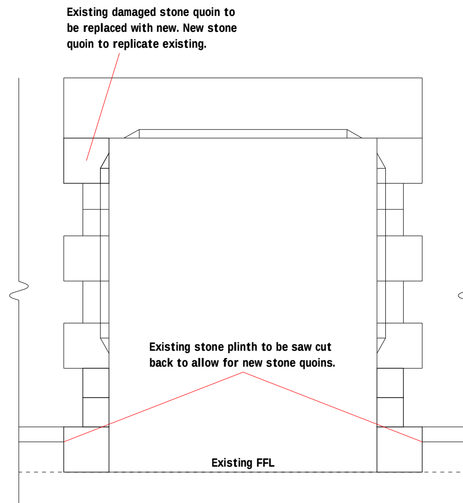
Proposed Opening - External View
