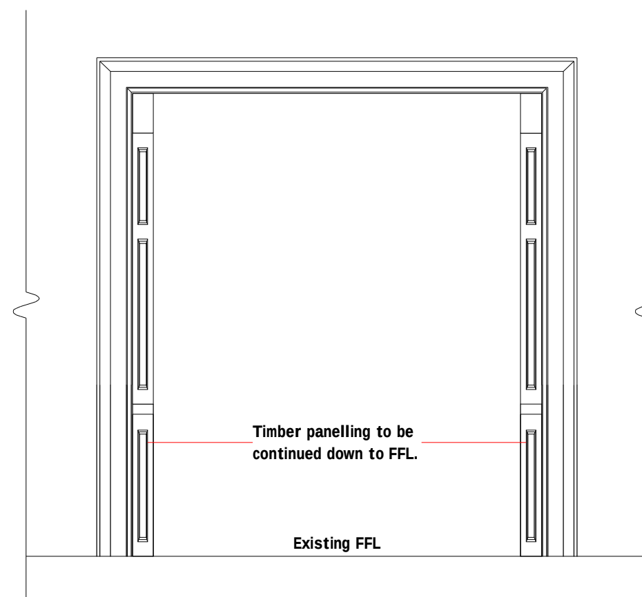
Proposed Opening - Internal View
