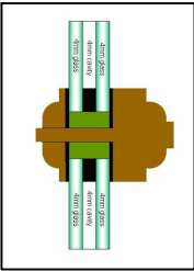
Glazing Bar Detail
