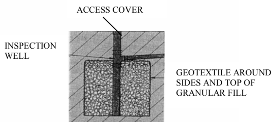
Fig 3 Small, filled soakaway with perforated inspection well to base of soakaway providing access to discharge drain outlet.
