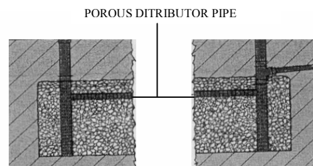
Fig 4 Trench-type soakaway with horizontal distributor pipe
