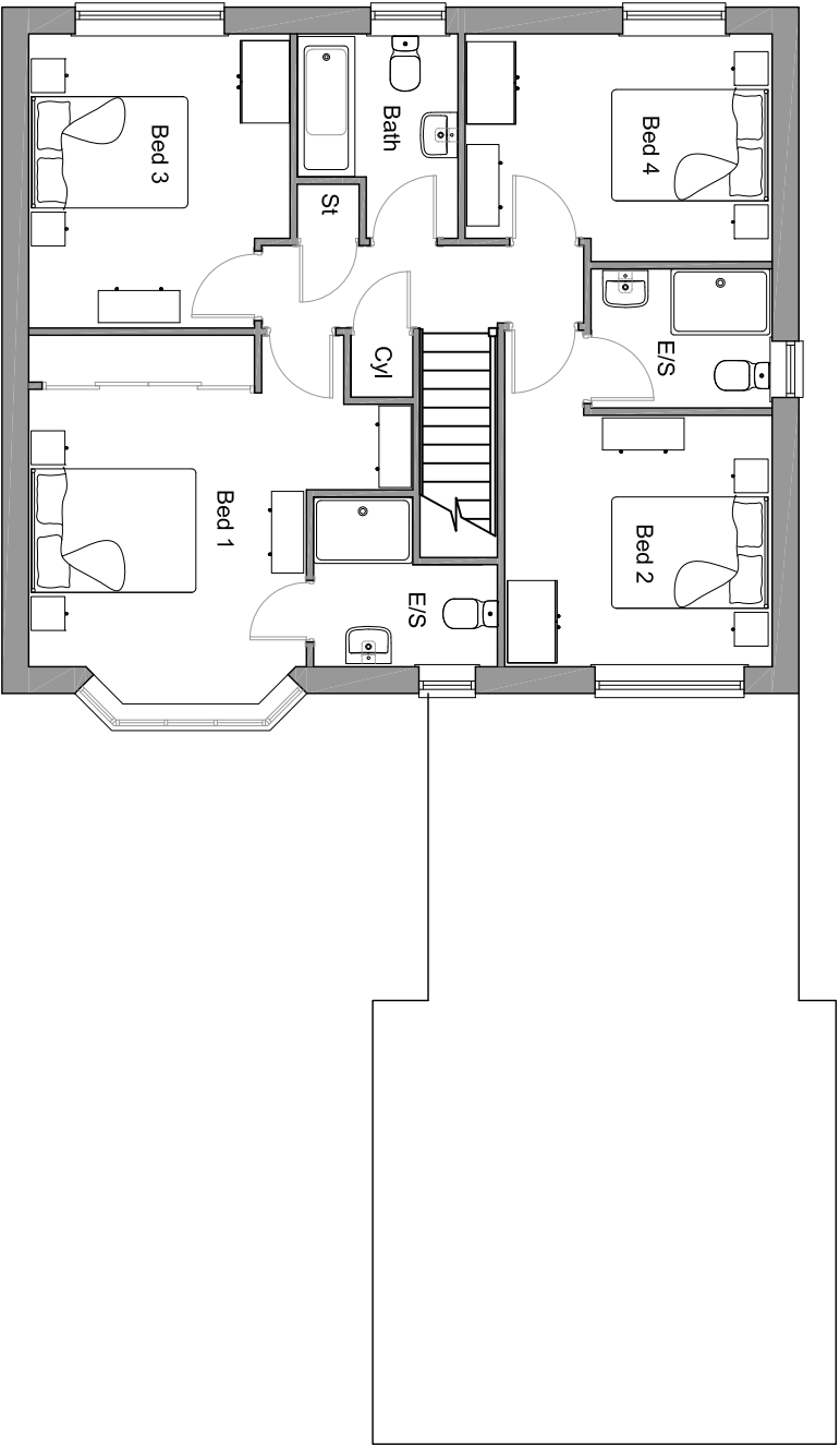
FIRST FLOOR
