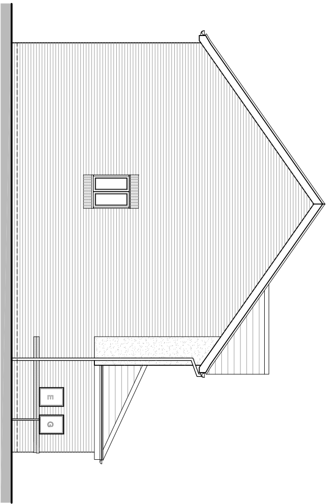
SIDE ELEVATION
