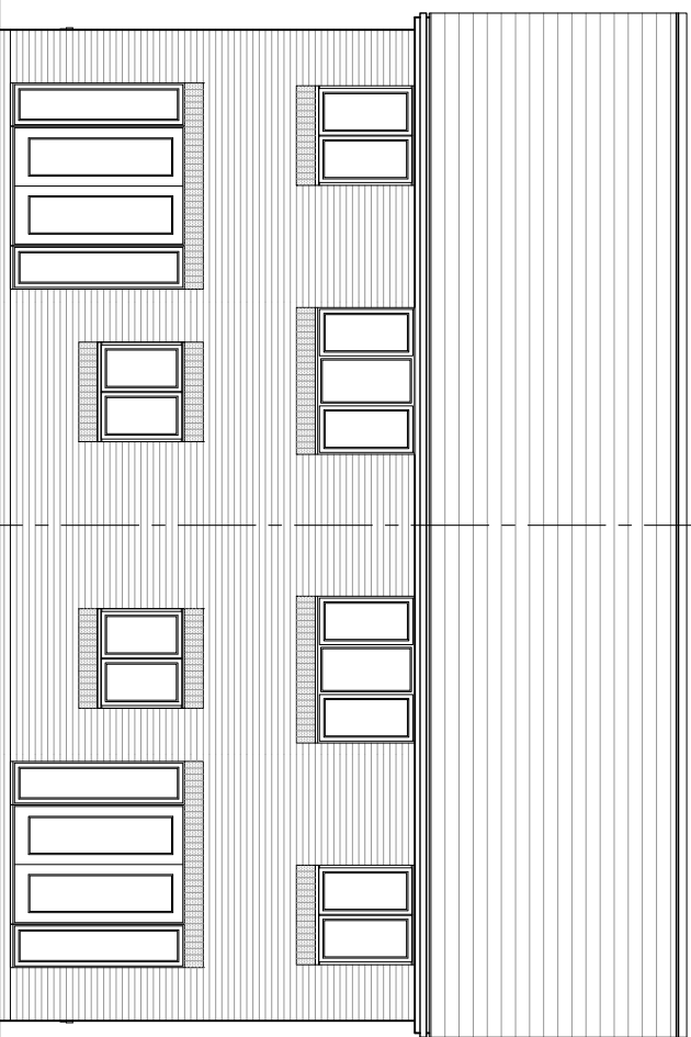
REAR ELEVATION
