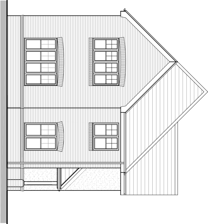
SIDE ELEVATION
