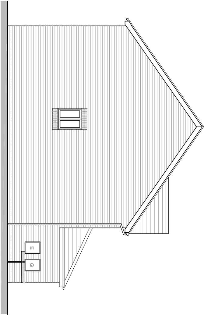
SIDE ELEVATION
