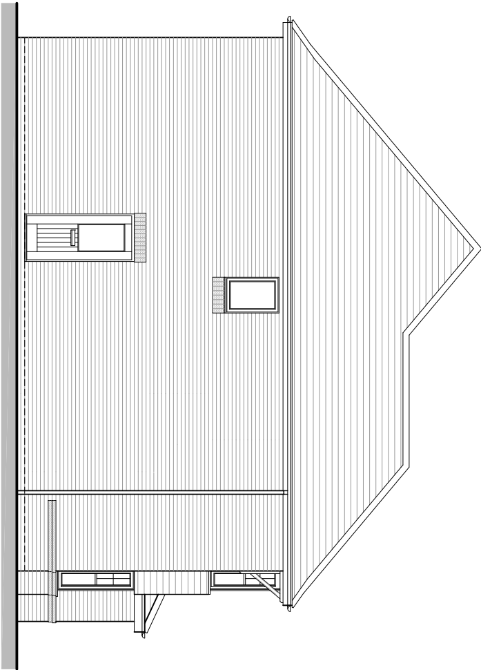
SIDE ELEVATION
