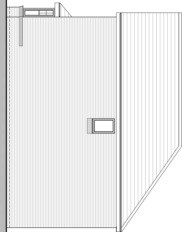
SIDE ELEVATION
