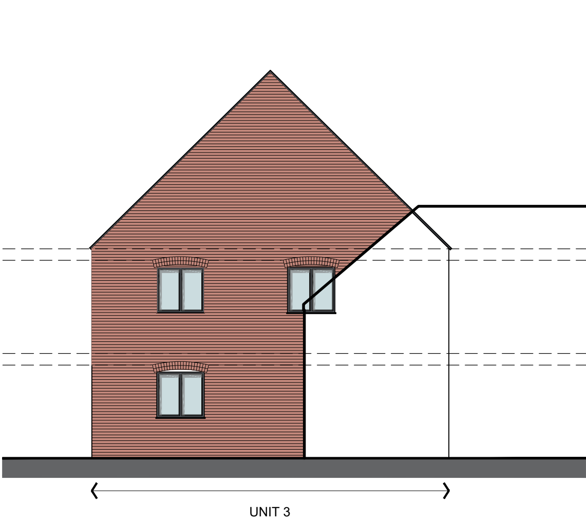
E10 Proposed Elevation Scale: 1:100
