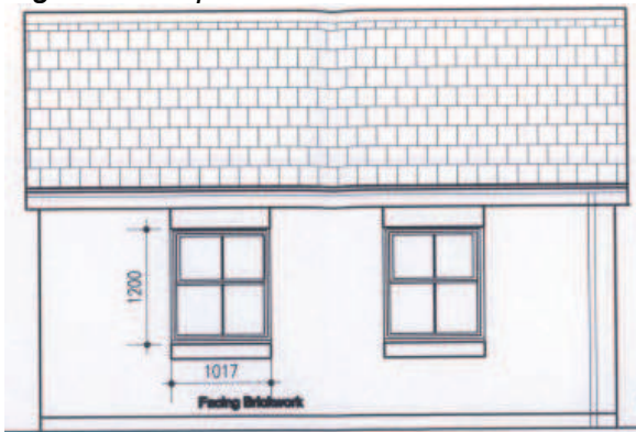
Figure 2. Proposed Rear Elevation
