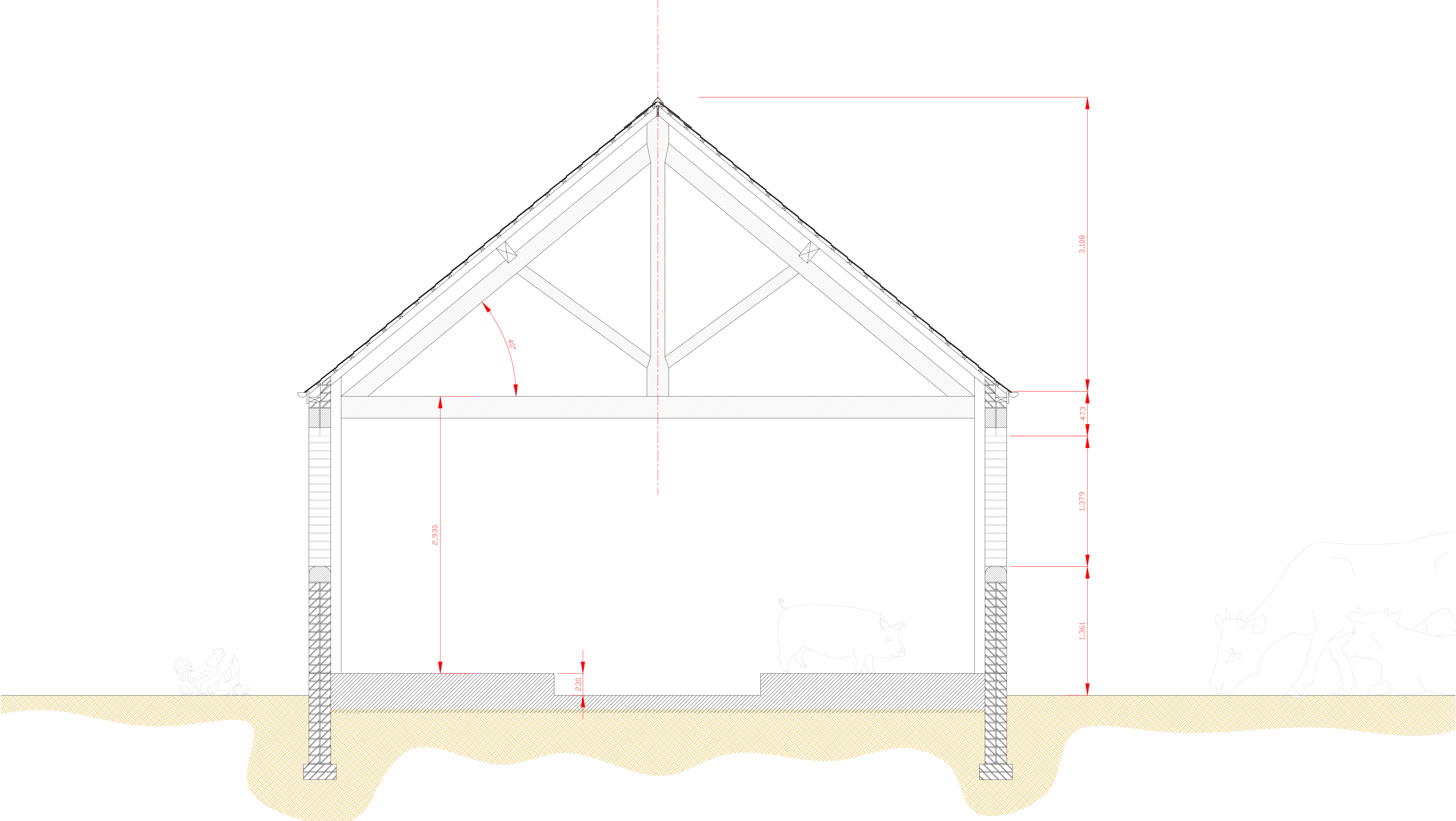
Typical Cross Section Through Main Barn Building Scale 1:20
