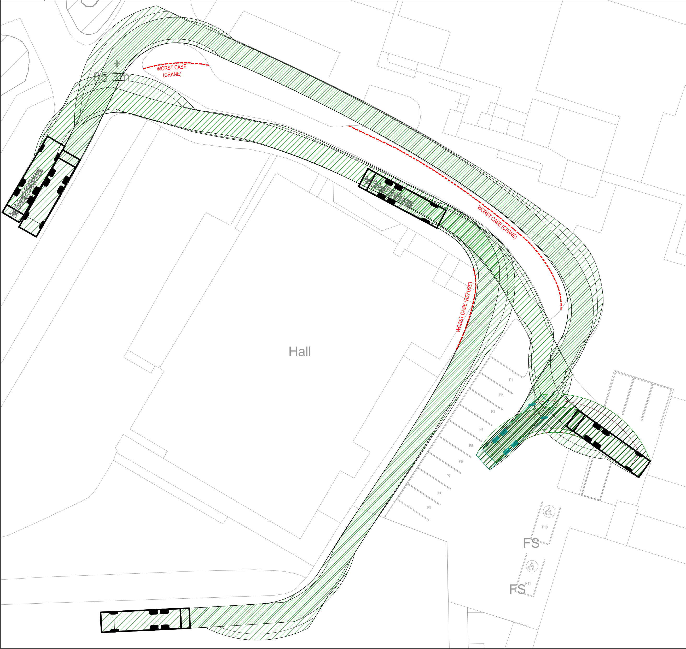
REFUSE VEHICLE
