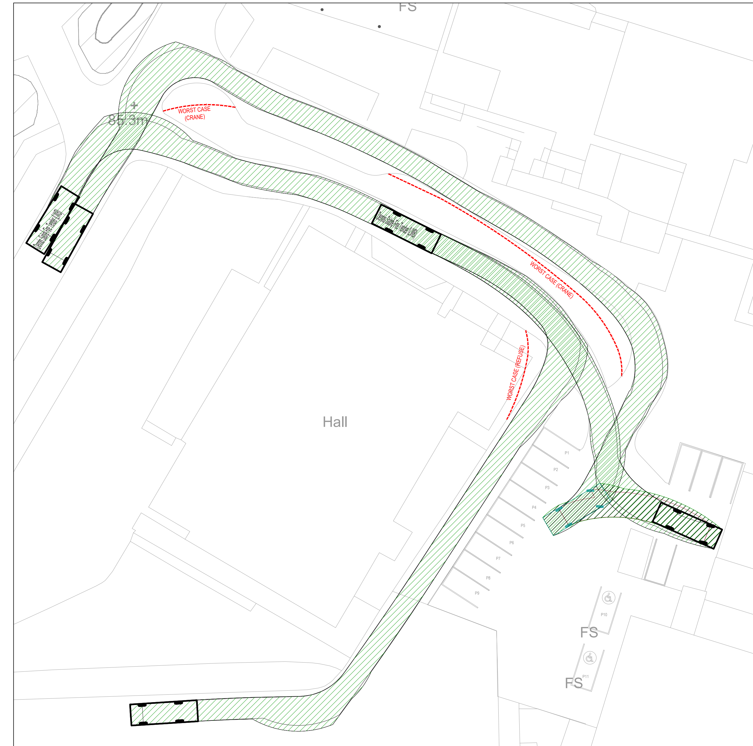
FIRE TENDER
