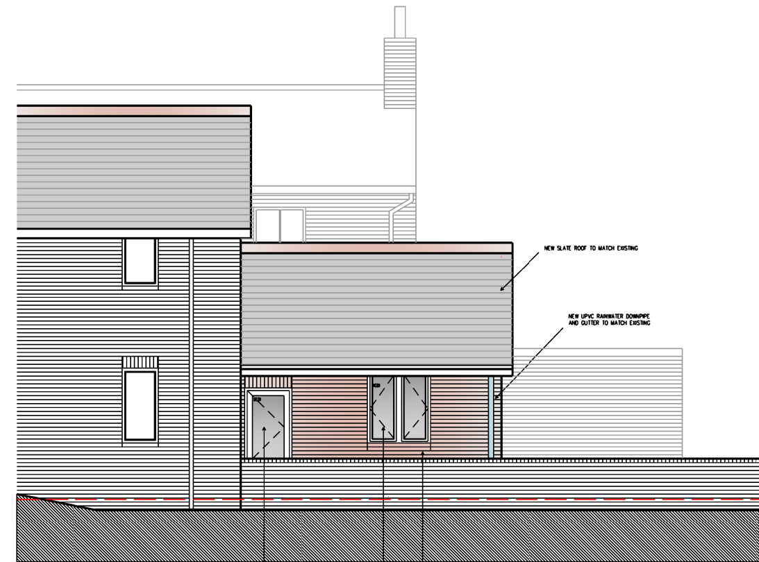
PROPOSED SOUTH ELEVATION 004
