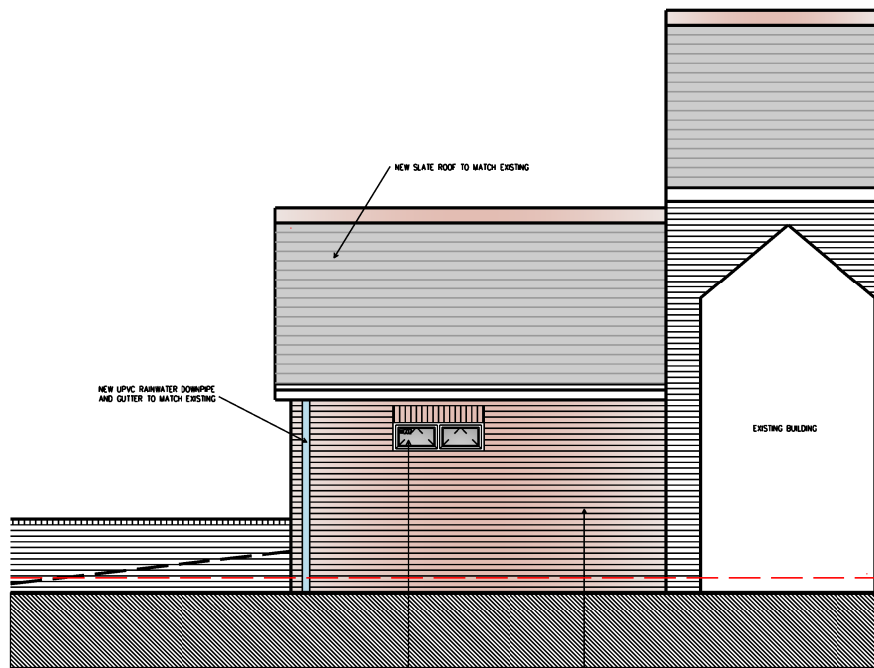
PROPOSED NORTH ELEVATION 005
