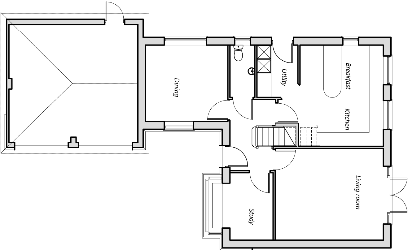
Ground floor layout plan Floor area excl garage: 66 sq m/710 sq ft 67.09 sqm/722 sq ft inclusive of bay
