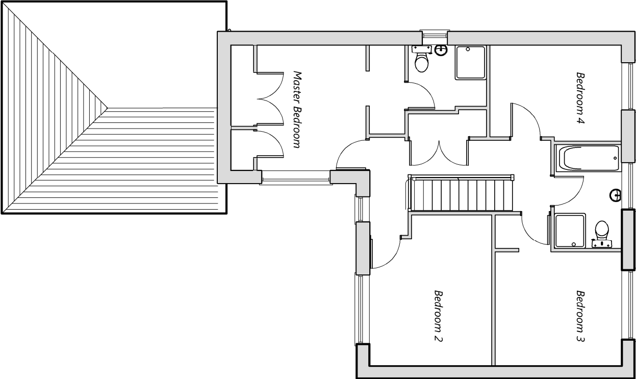
First floor layout plan Floor area: 66 sq m/710 sq ft
