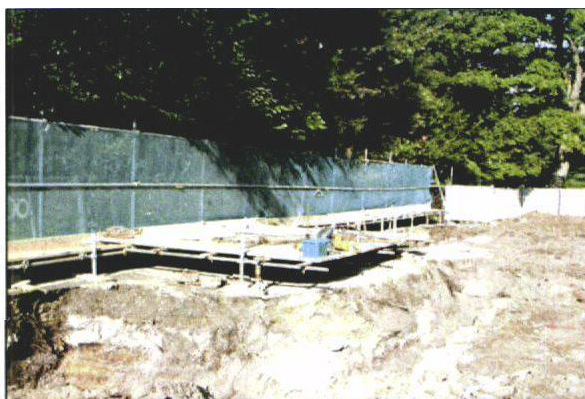
Photo 10: A scaffold framework attached to the main scaffold fencing can be used to support either scaffold planks or plywood to create an elevated platform with a gap beneath.
