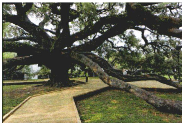
Photo 31: Board walks supported on posts or a light frame are another way of providing pedestrian access across sensitive RPAs.
