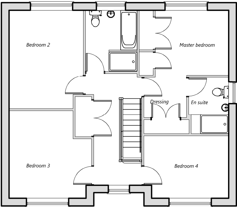
First floor layout plan
