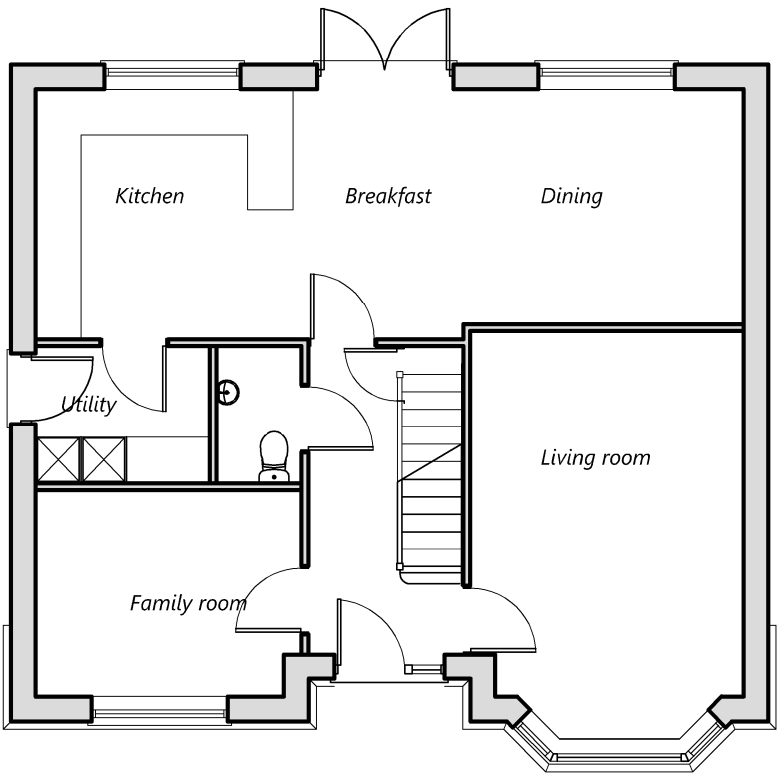
Ground floor layout plan
