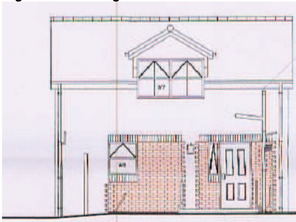
Figure 2. Proposed Front Elevation
