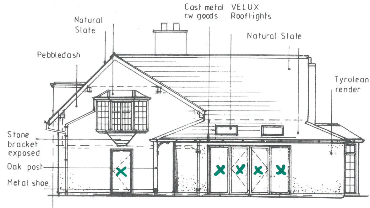
WEST ELEVATION
