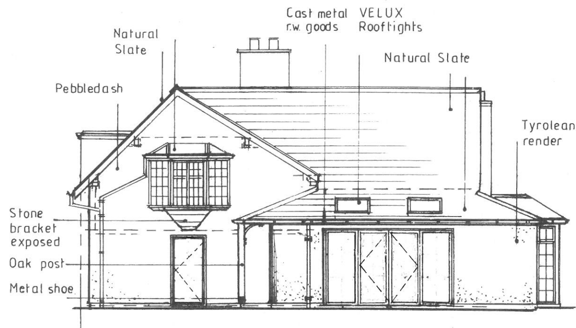
WEST ELEVATION
