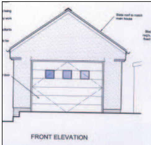
Proposed Garage
