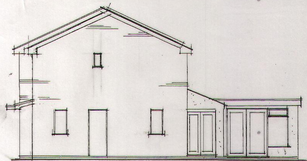
SIDE ELEVATION
