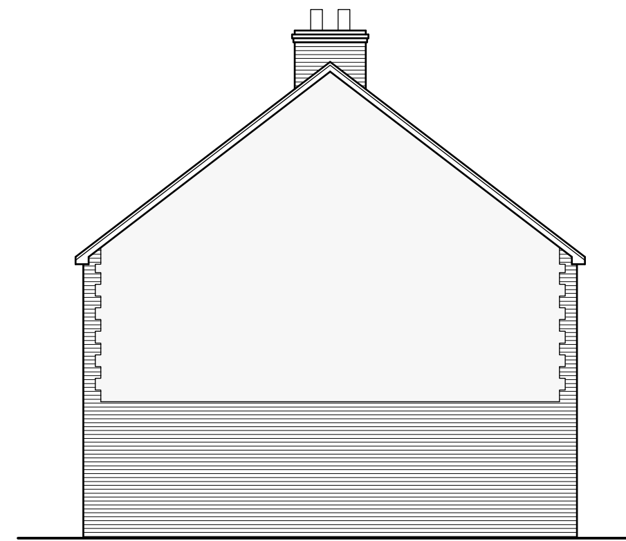
Side Elevation
