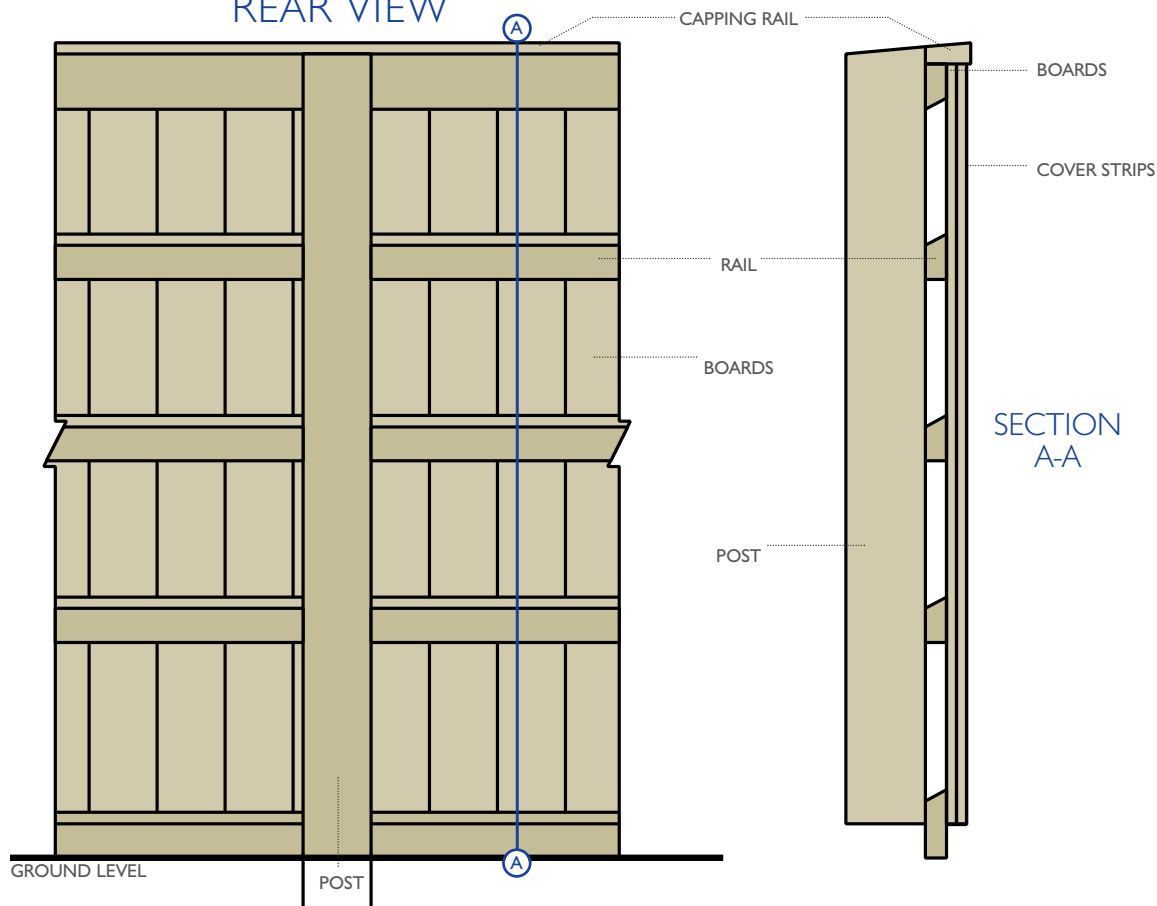
REAR VIEW
