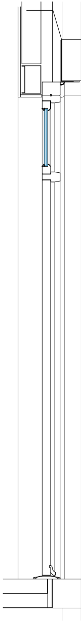
Typical Section
