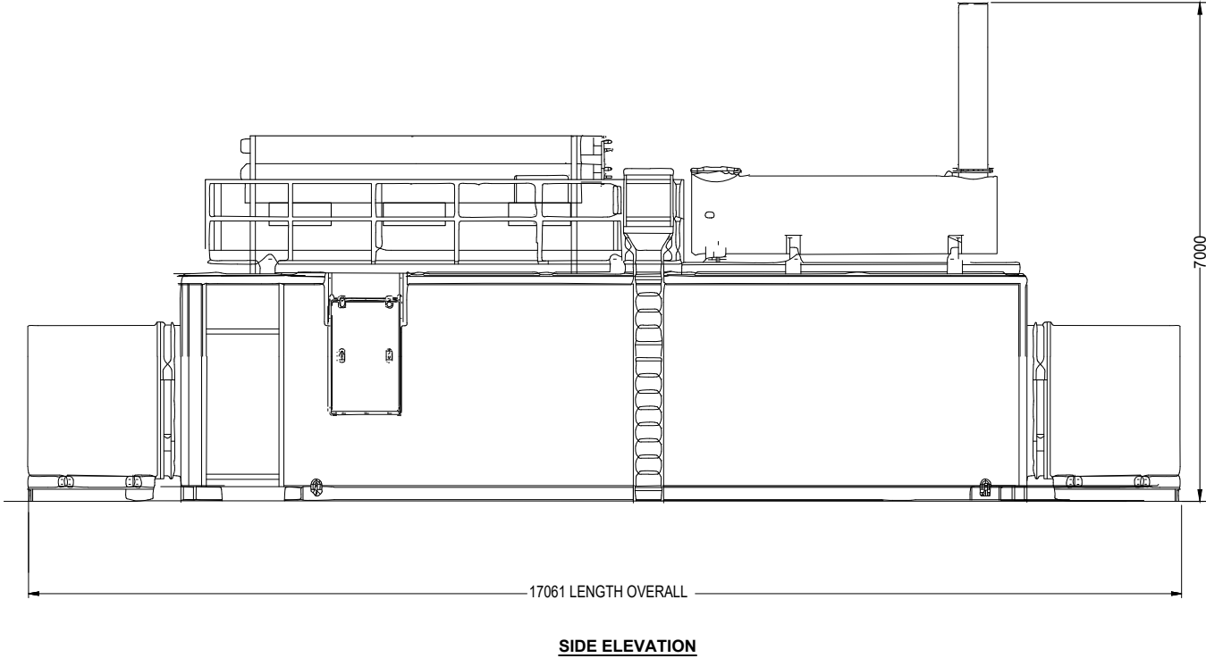
ROOF MOUNTED COMBINED JACKET/INTERCOOLER DRY COOLER
