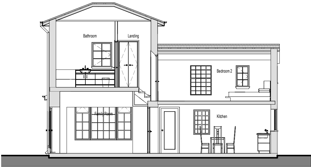
Proposed Section 1 1 : 100
