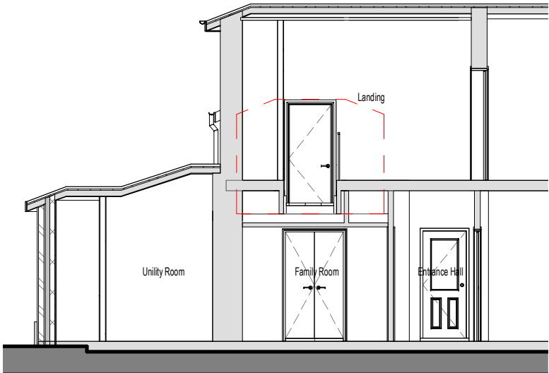
Proposed Section 3 1 : 100
