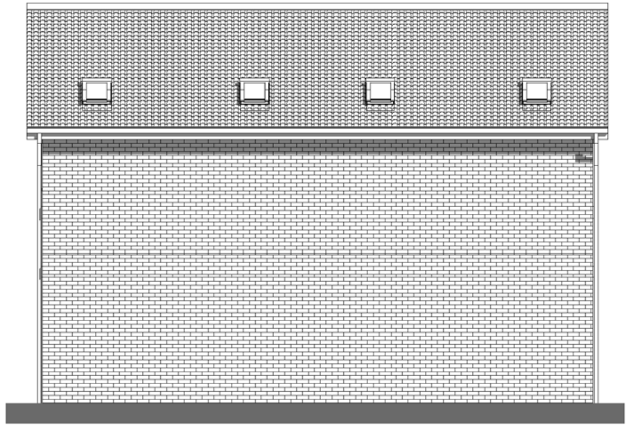
2 South Facing 1 : 100
