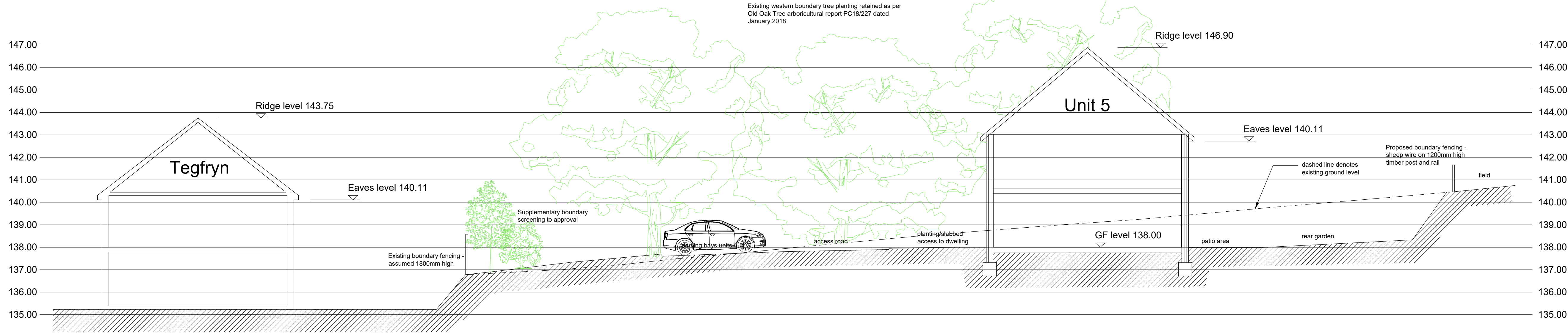
PROPOSED NORTH WEST / SOUTH EAST SITE SECTION SHOWING RELATIONSHIP OF NEW DEVELOPMENT WITH EXISTING DWELLINGS
