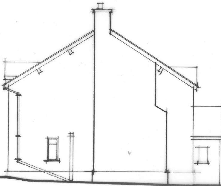
PROPOSED WEST GABLE ELEVATION 1.100
