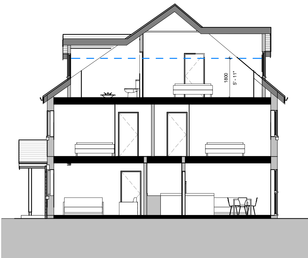
Section 2
