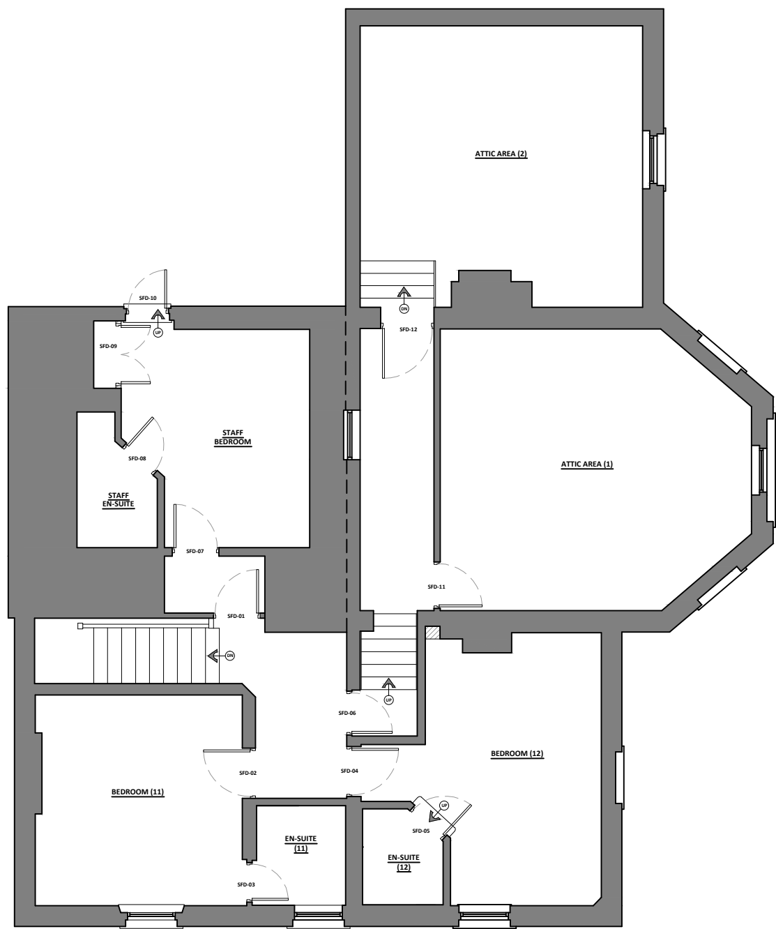
ARCINV227 THE WYNNSTAY ARMS, RUABON. 2ND FLOOR GENERAL ARRANGEMENT PLAN.
