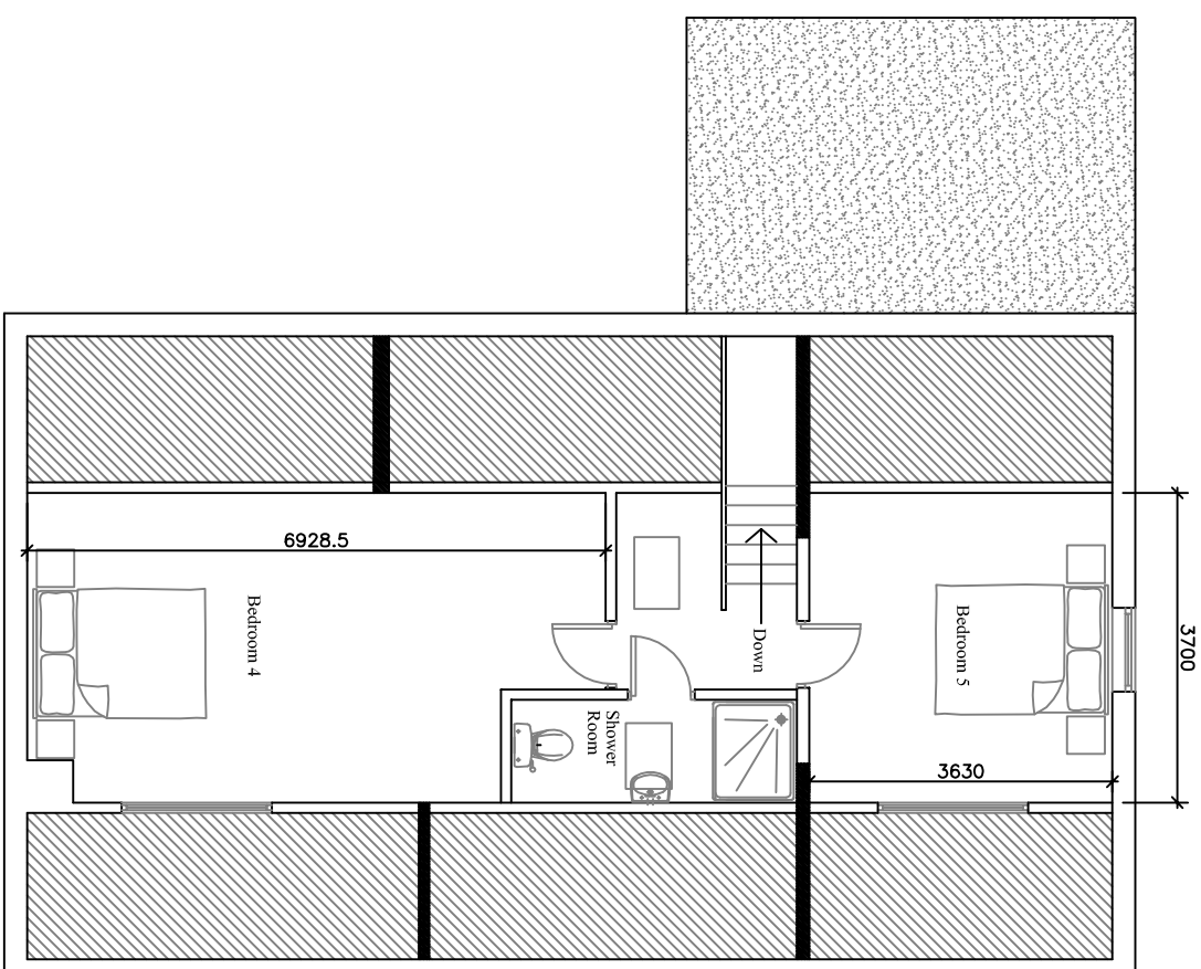
ATTIC FLOOR PLAN
