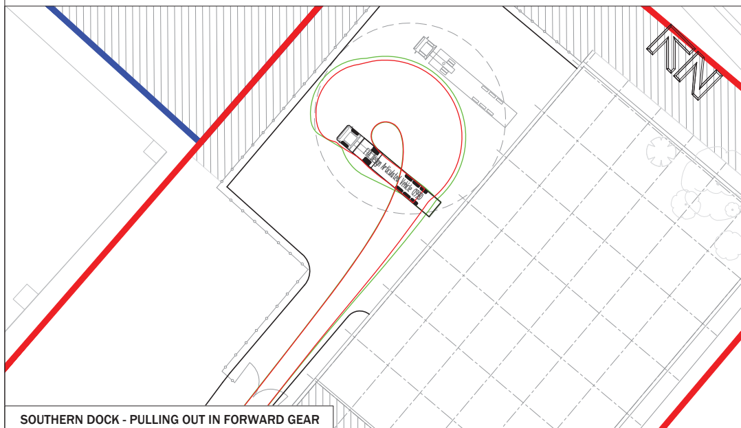
SOUTHERN DOCK - PULLING OUT IN FORWARD GEAR
