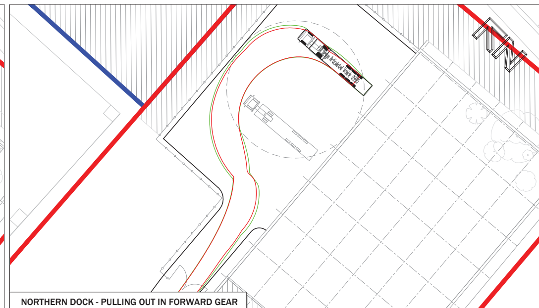
NORTHERN DOCK - PULLING OUT IN FORWARD GEAR
