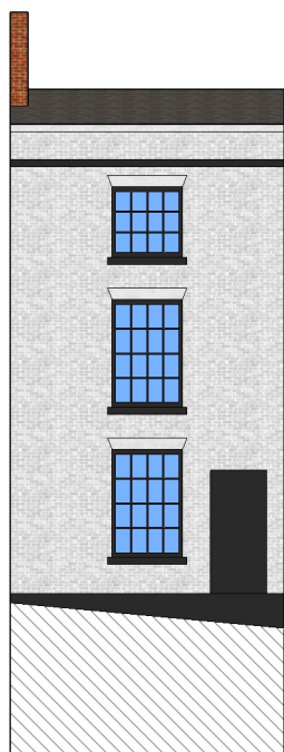
Proposed Front
