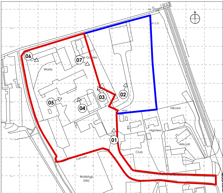
KEY PLAN [1:2500]
