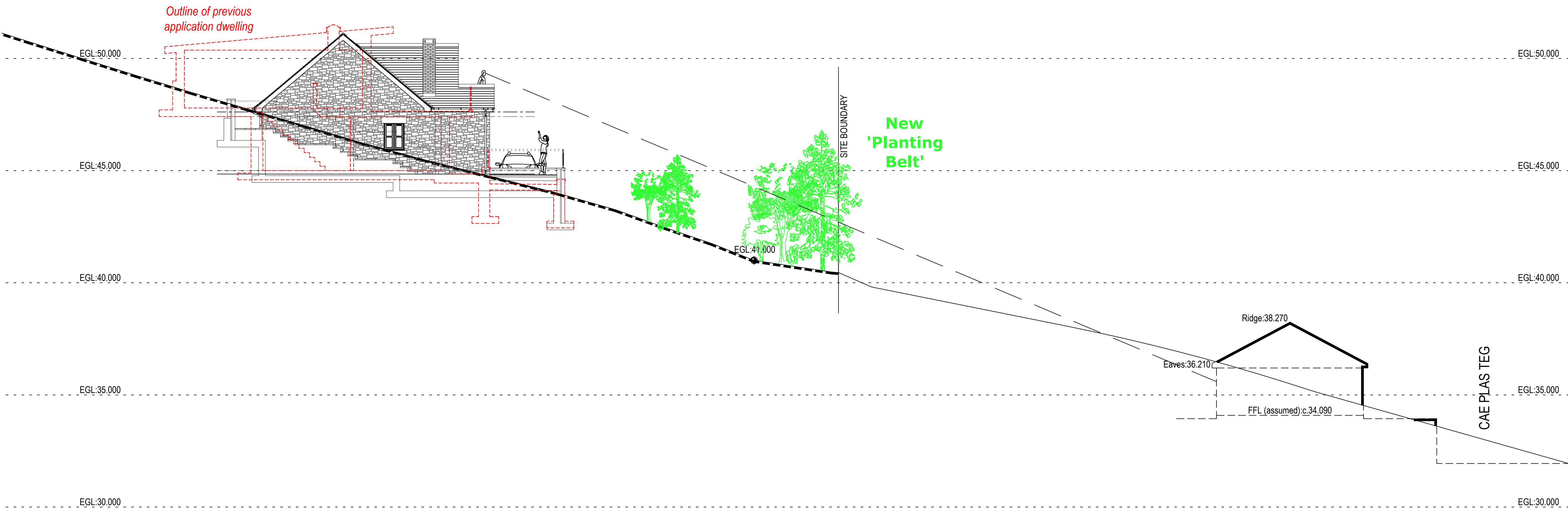
SITE CROSS SECTION B-B: BASIC SITE CROSS SECTIONS: 1:100(A1)
