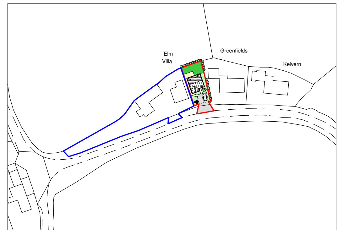
Location Plan 1:1250
