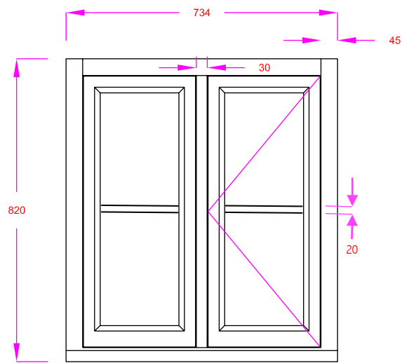
DORMER WINDOW ELEVATION PONTRICKETT Scale 1:10
